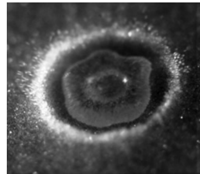
Fig. 1 Granular impact cratering by a water droplet.
